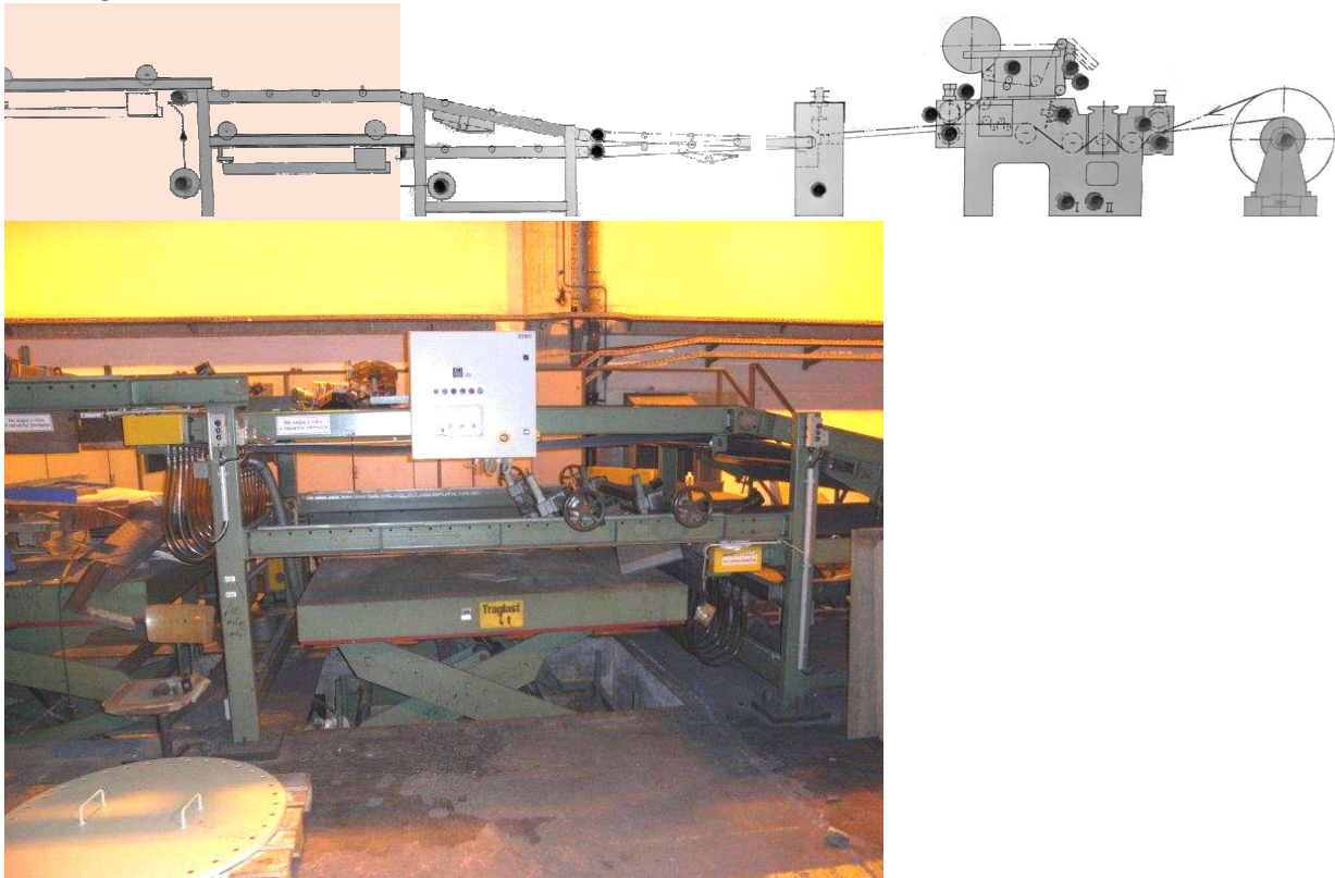
Stacking table
